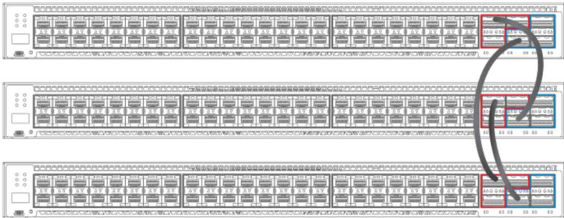
FIGURE 39 ICX 7750 ring stack from rear panel
