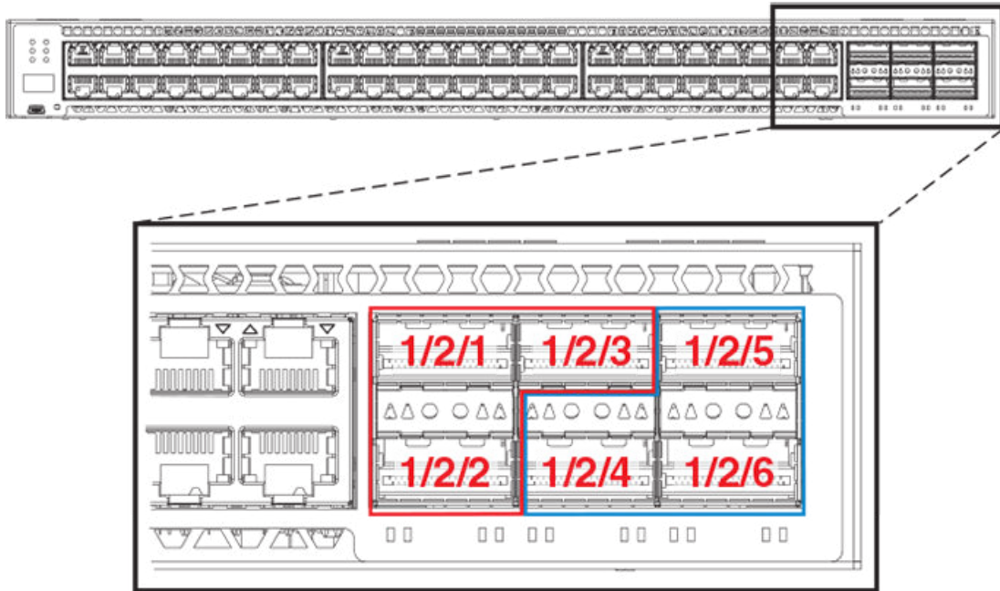
FIGURE 34 ICX 7750 stacking ports on front panel
